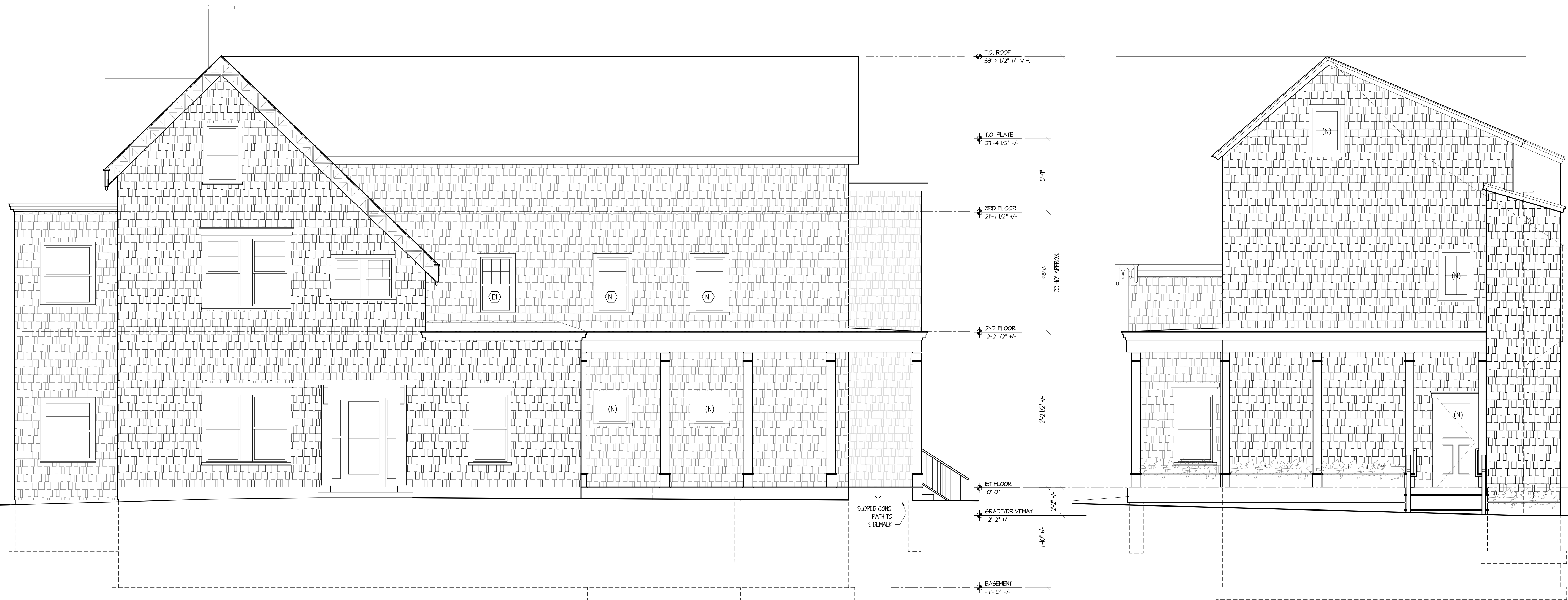
1 NORTH ELEVATION 1/4"=1'-0"
